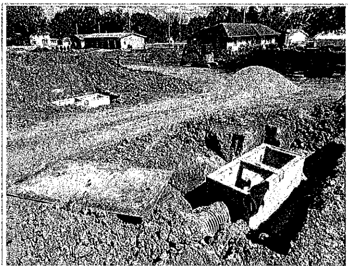
Storm sewer structures installed at north side of Rose and 3rd Street, structures also installed at west side of same intersection
