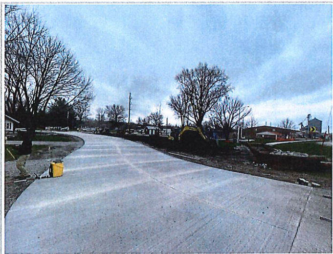
NE corner of site looking SW. Newly saw cut Hickory street.
